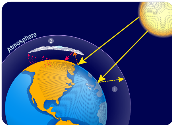
Figure 22.4 Global warming
