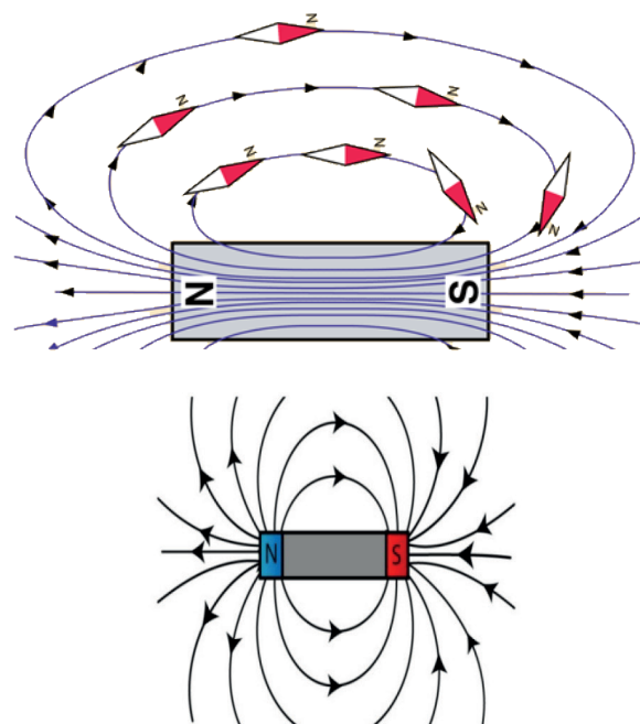
Figure 7.4 Magnetic Field
