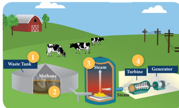
Figure 15.8 Bio-gas
