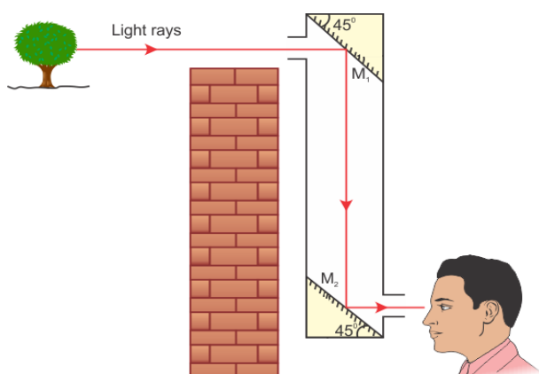
Figure 3.10 Periscope
