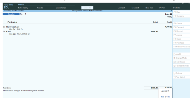
Figure 11.3.2 Receipt Voucher entry for maintenance charges due for the previous year received from Narayanan
